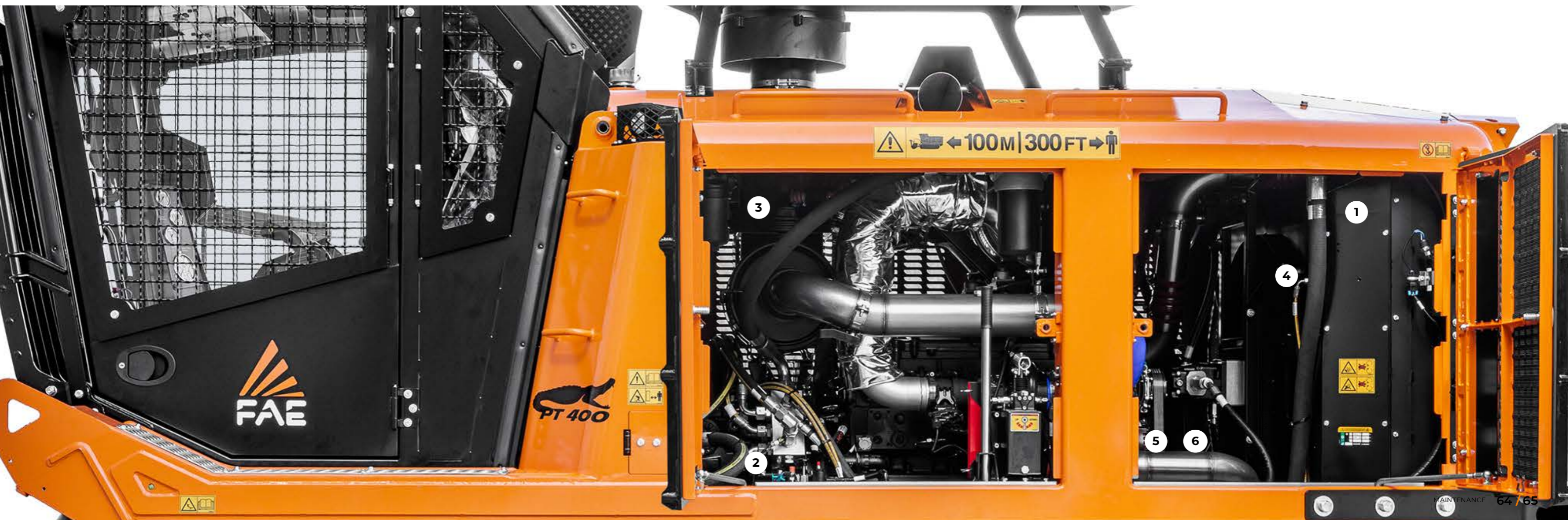
Level control is simplified by an organized layout (1)
