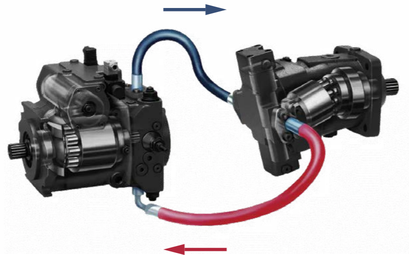
Diagram of the FAE PT200 hydrostatic transmission : simple and effective
